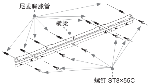
螺钉 ST8×55C
